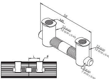
CONECTOR DE PERFILES "ALUSKIT®"
